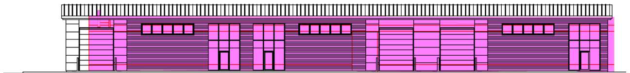
FRONT ELEVATION (with existing building overlay shaded pink)
