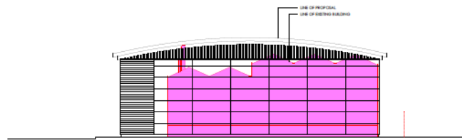
SIDE ELEVATION (with existing building overlay shaded pink)
