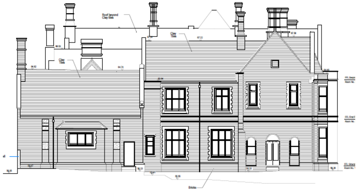
ELEVATION D South Elevation
