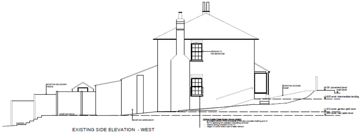
EXISTING SIDE ELEVATION - WEST
