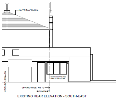
EXISTING REAR ELEVATION - SOUTH-EAST
